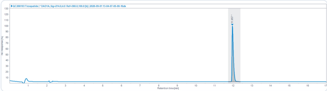
HPLC Chromatogram · Retention Time 11.957 min
